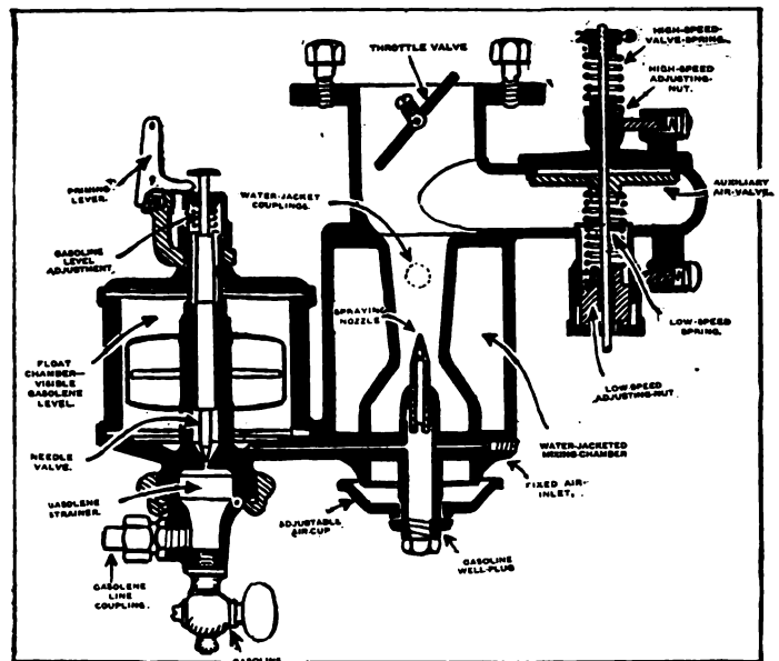
A Typical Modern Carbureter Shown in Section.
